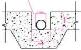
INLET CHANNEL IN POOL FLOOR
